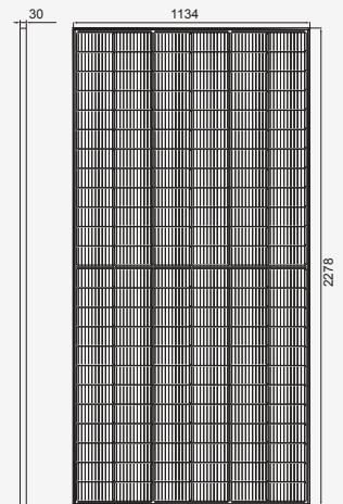
Vista Frontal
